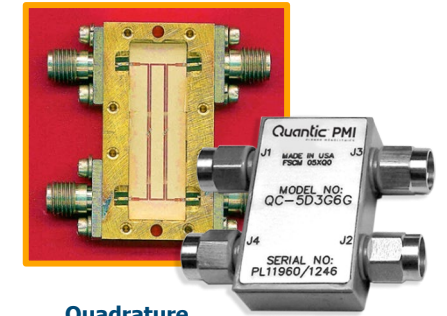
Quadrature Couplers
